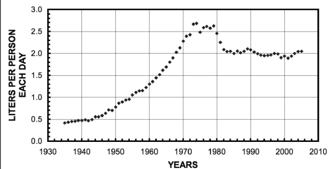
Fig. 2: WORLD PER CAPITA PRODUCTION OF CONVENTIONAL PETROLEUM Production data from Colin Campbell
