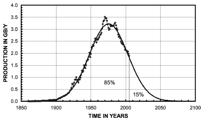
FIG.1: US OIL PRODUCTION
